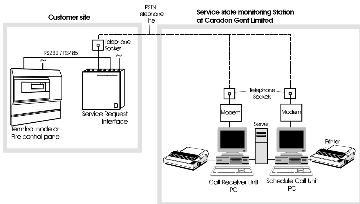
Figure F-2 System wiring
