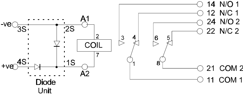
Figure 65-5 Relay connections
