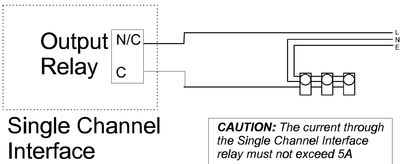
Figure 18-1 Door release interface circuit
